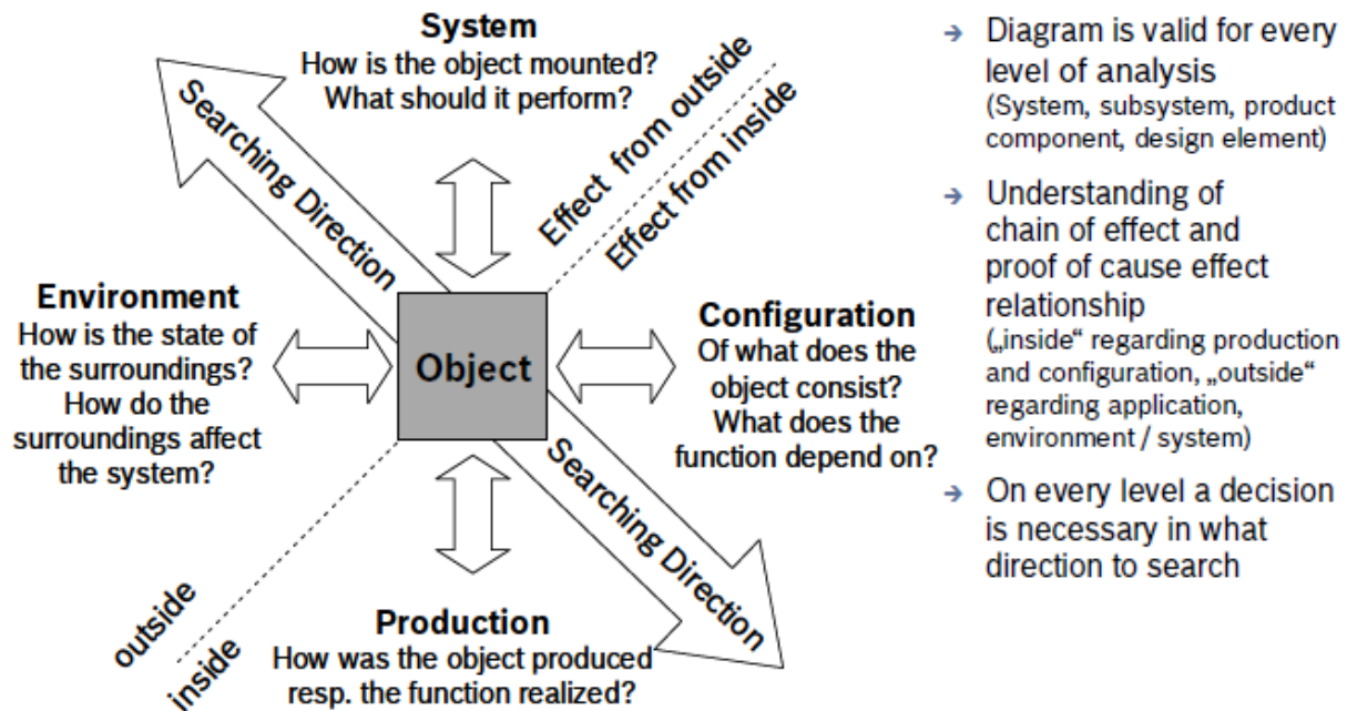
Figure 5.8: Directions of investigation for resolving product problems
